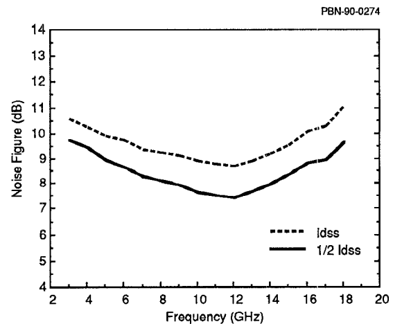
Figure 7. Receive Noise Figure of the T/R Circuit.
