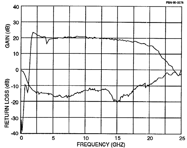
Figure 6. Receive Gain and Return Loss of the T/R Circuit.
